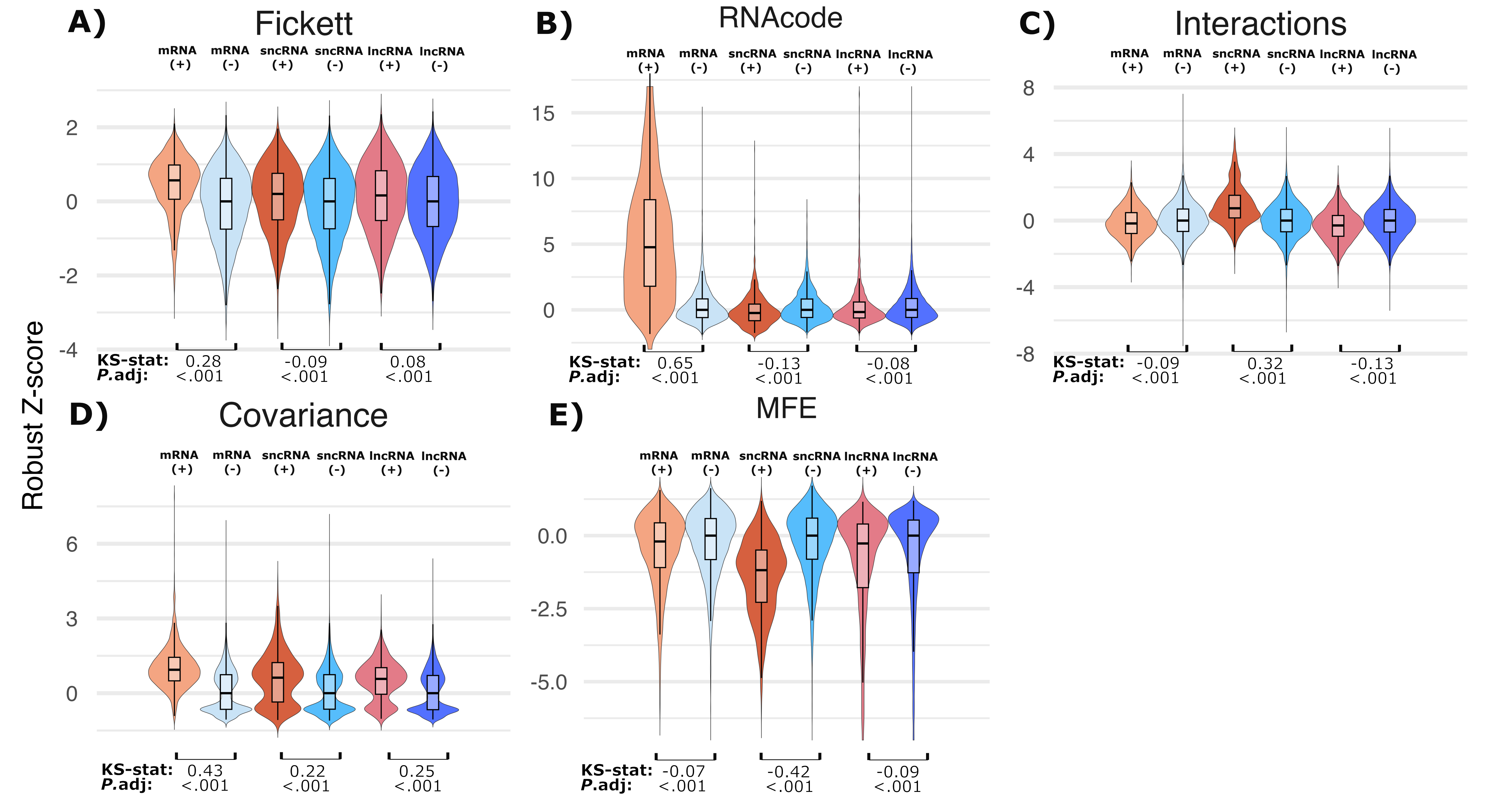
Figure 5. Violin plot and box plots for the distribution of mRNA and ncRNA specific features based on robust z-scores for genic and matched non-genic regions. A&B) Fickett and RNAcode, coding potential based on a measure of nucleotide composition bias and positional asymmetry/ or evolutionary signatures of purifying selection on synonymous sites within multiple sequence alignments, respectively. C) Interactions, average interaction free energies between sequences and 34 abundant human ncRNAs from RNACentral. D) Covariance, measure of evolutionary pressure to maintain RNA base-pair interactions, reflecting structural constraints. E) MFE, lowest thermodynamic energy of the most stable predicted RNA secondary structure. Signed Kolmogorov-Smirnov statistics and adjusted p-values are displayed under each comparison.
